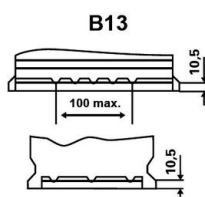
Hold Down
